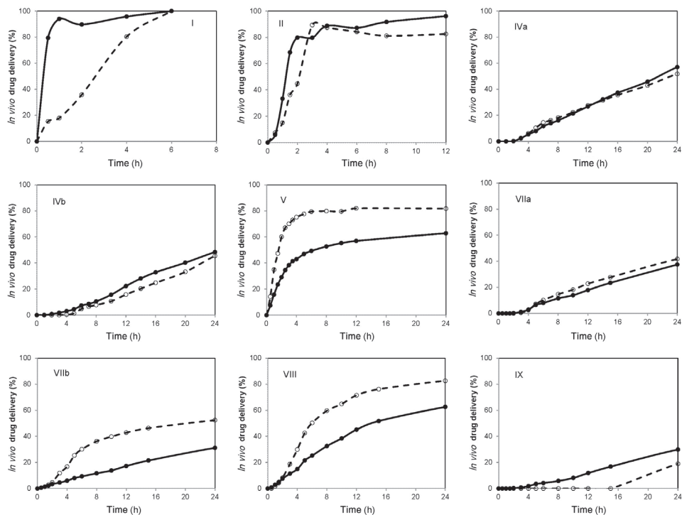
Fig. 2. In vivo drug delivery profiles of various nifedipine products administered in the fasted (full line) or fed state (dotted line) obtained by numerical deconvolution with oral reference. See Table I for key to legend.
