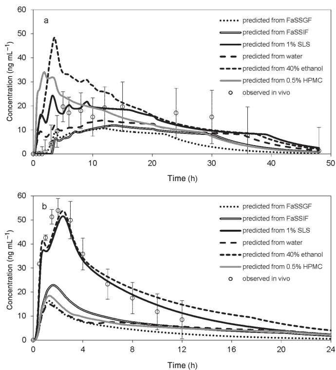
Fig. 4. Plasma concentration profiles of: a) osmotic controlled-release tablets and b) hydrophilic matrix tablets predicted using the GastroPlus™ model under fasting condition.
