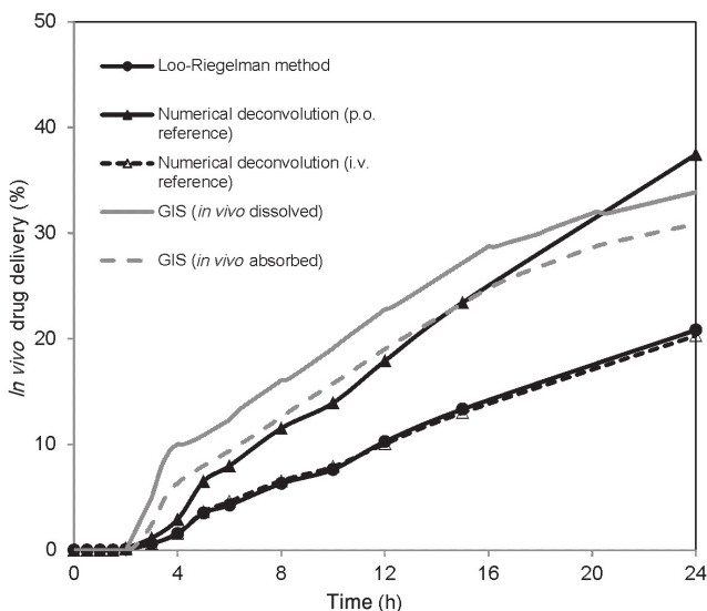
Fig. 1. Nifedipine in vivo delivery profiles of osmotic controlled-release tablets under fasting conditions estimated by different methods.
