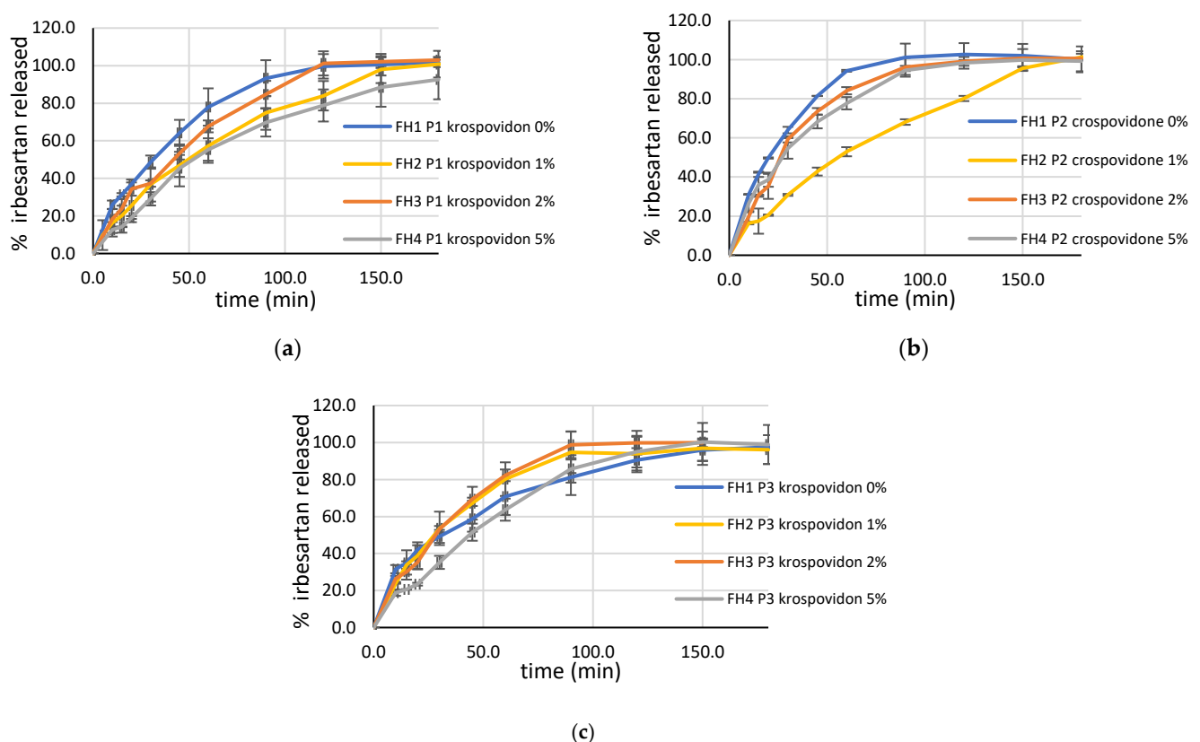
Figure 10. Effect of crospovidone on drug release: (a) tablets printed with a laser speed of 100.00 mm/s; (b) tablets printed with laser speed of 120.00 mm/s; (c) tablets printed with laser speed of 140.00 mm/s.
