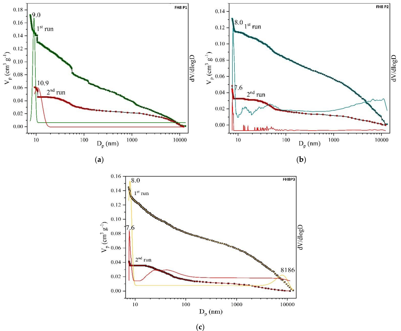
Figure 5. Pore size distribution curves of SLS tablets (a) FH8 P1, (b) FH8 P2, and (c) FH8P3.
