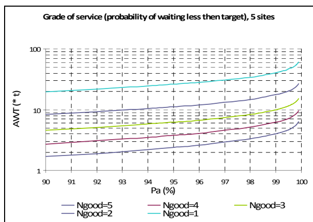
Figure 3. Grade of Service: probability ( P_a (%)) that waiting time is smaller than the predefined target value ( AWT ), AWT expressed as a multiple of base time interval ( t ); number of the experienced technicians ( N_{good} ) is parameter for the characteristics
