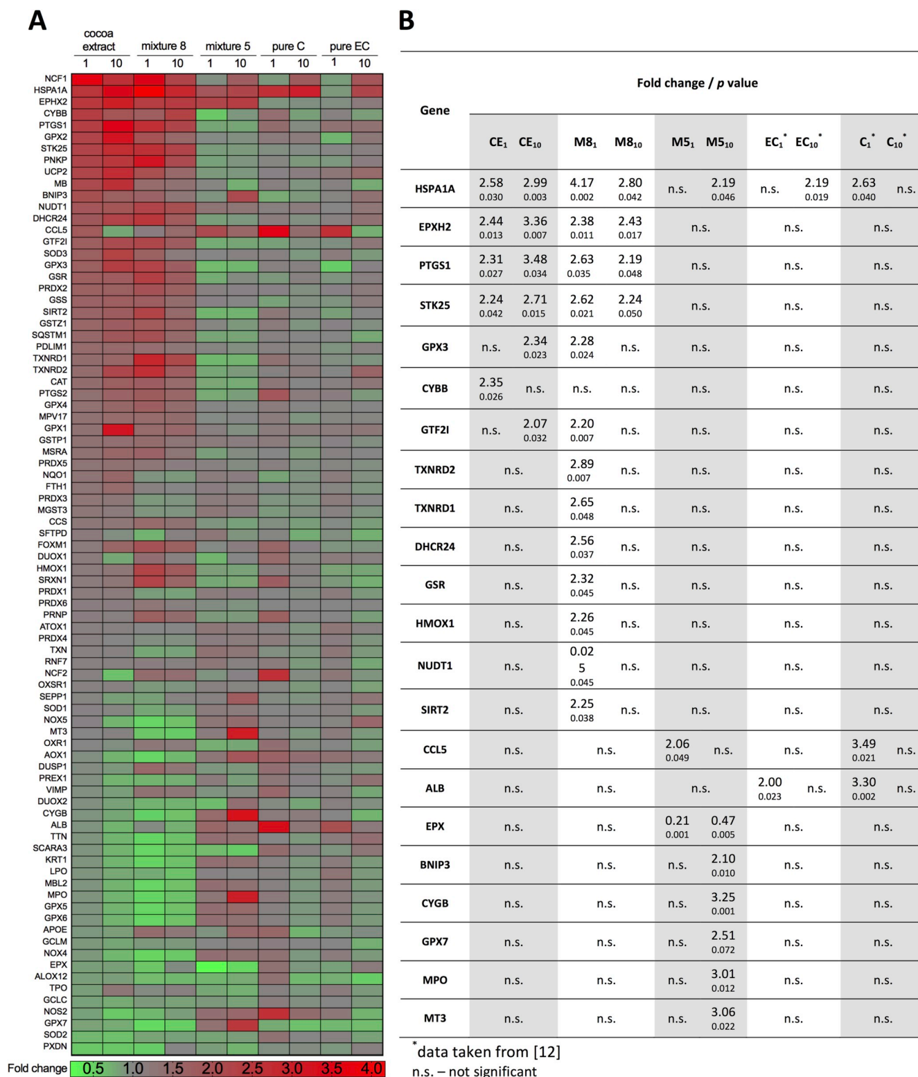
Fig. 6. A – Heat map presenting the modulation of 84 oxidative stress response and antioxidant defence genes in HT29 cells after 24 h treatment with CE and two model mixtures M8 and M5 at concentrations of CEC amounting to 1 or 10 μM, as well as pure catechins EC and C at concentrations of 1 or 10 μM. B – statistically significant changes in the expression of genes as a result of indicated treatment. The results are calculated based on three independent experiments.
